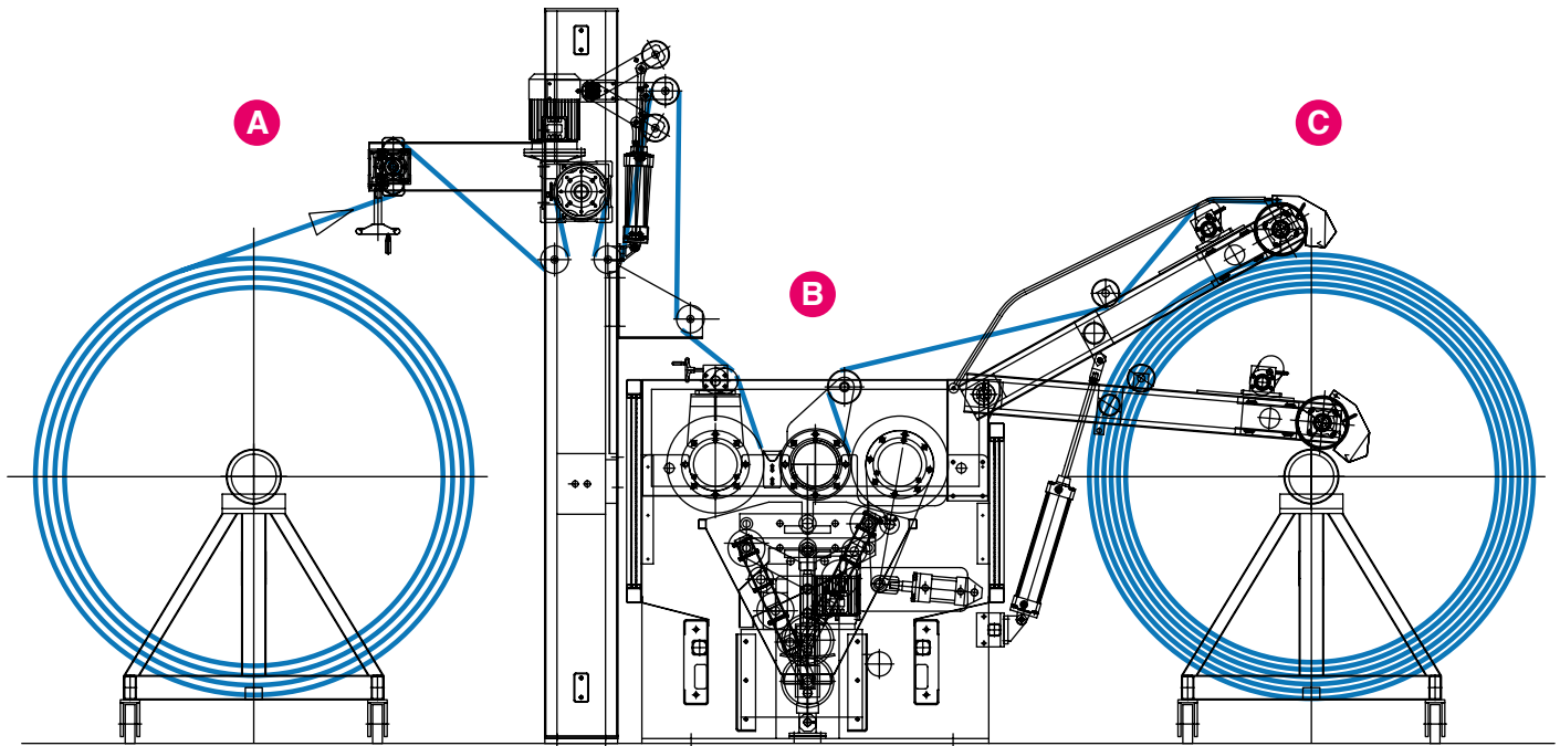
A Entrata grande rotolo Entry frame for rolled batch
