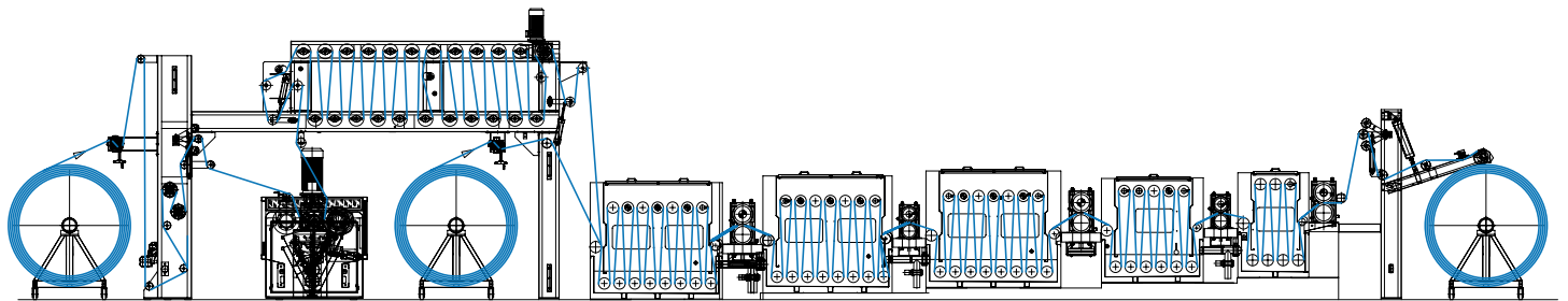
A Sodatrice / mercerizzatrice in continuo con lavaggio Causticizing-mercerizing machine in line with washing machine
